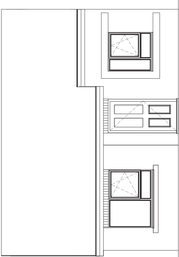
Front Elevation 1 : 50
